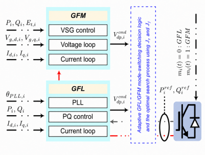
Figure 2: Switchable controller branches.
