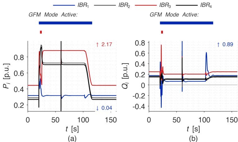
Figure 8: Active and reactive power per converter
