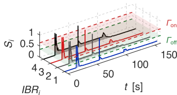
Figure 5: Severity index S_i per converter.
