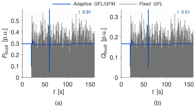
Figure 10: Bus-9 active and reactive power: adaptive vs locked-GFL diagnostic.
