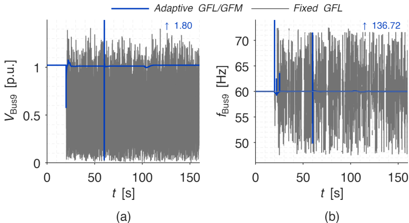
Figure 9: Bus-9 voltage and frequency: adaptive vs locked-GFL diagnostic.
